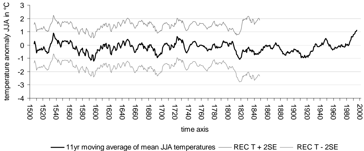
Figure S5 | 11-year moving average of mean summer (JJA) temperatures for central Europe (1500–2000) Data from Dobrovolný et al. 2010, kindly supplied by the main author.
