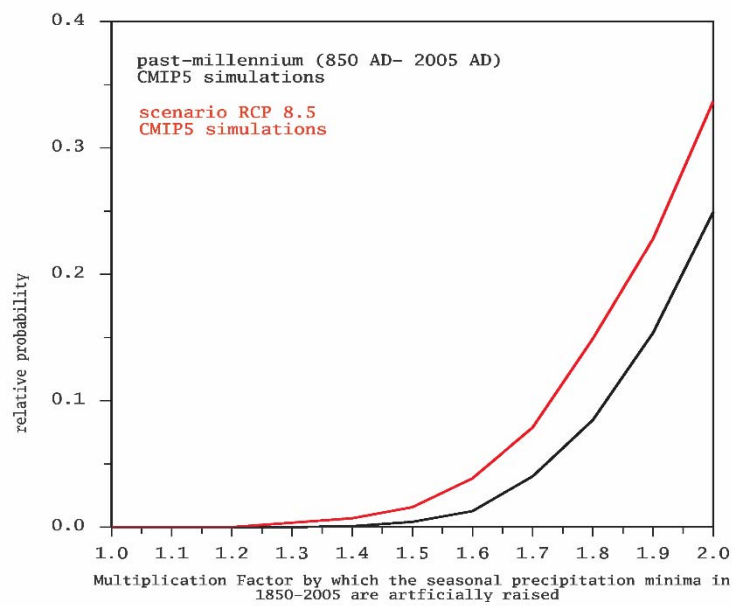
Figure S4 | Relative probability of occurrence of extreme drought years. Assessed over spring, summer and autumn Central European precipitation in 1540 is simultaneously lower than the (re-scaled) simulated seasonal minima of the AD 850–2005 period. Simulations comprise six past-millennium simulations from the CMIP5 model suite (black line) and six scenario simulations (scenario RCP8.5) until AD 2100 with the same models.
