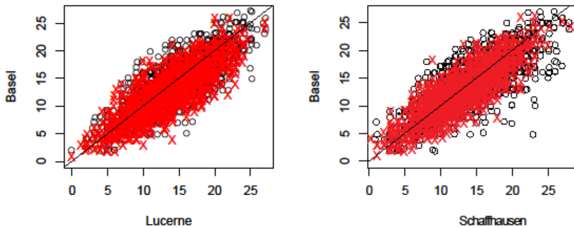
Figure S3 | Scatter plots of days with precipitation (NRD) during the instrumental period, 1864 – 2012. Circles = NRD \geq 3mm precipitation amount; crosses = NRD \geq 1 mm precipitation amount
