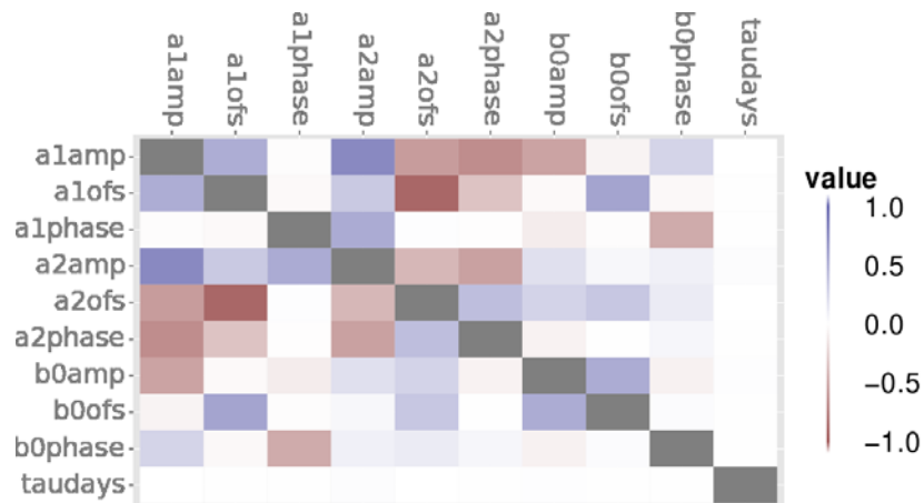
Figure S2 | Cross correlation between the draws of the parameters for WCEu
