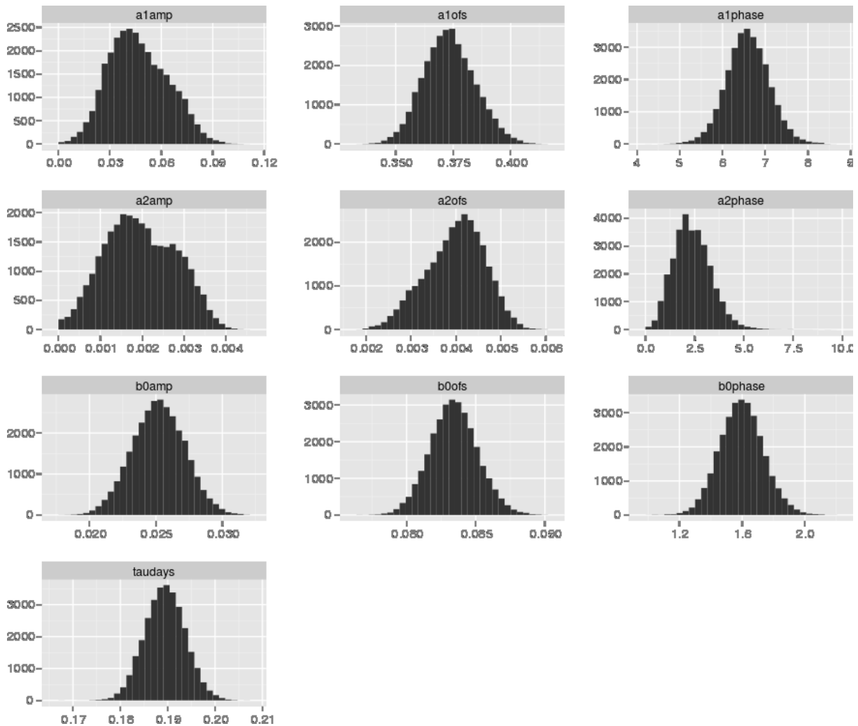
Figure S1 | Draws of the model parameters for WCEu for all chains. Top and second row: parameters for the scale a1 and a2, third row: parameters for the shape b0. Bottom figure: draws for the spread in observations between different stations.
