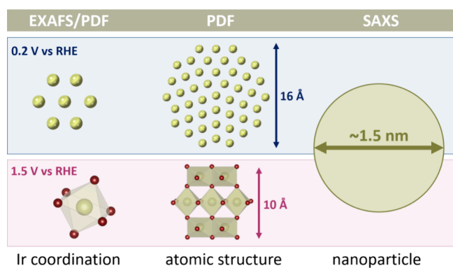
Figure 5. Sketch illustrating the information that can be extracted by operando X-ray PDF and SAXS on the structure of the electrochemically formed iridium oxide, which is active for OER. While PDF can provide information on the very local Ir–O and Ir–Ir coordination similar to EXAFS, PDF can also provide information on the arrangement of metal polyhedra within the nanoparticle. Combined with morphological information from SAXS, a complete picture of the atomic structural arrangement in the iridium oxide nanoparticle is obtained.
